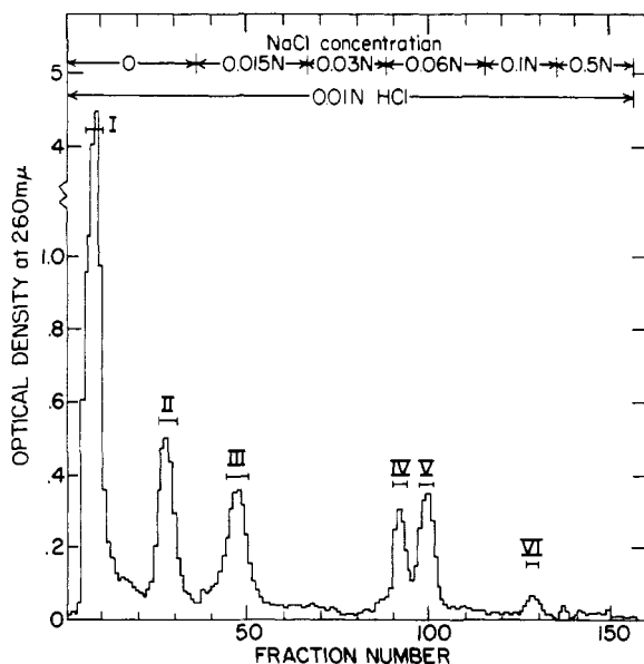
FIG. 1.—Separation of Porphyra perforata nucleotides by anion exchange chromatography on a Dowex 1 ( \text{Cl}^- ) column. The nucleotides were eluted with 0.01 N hydrochloric acid containing increasing concentrations of sodium chloride as indicated.
